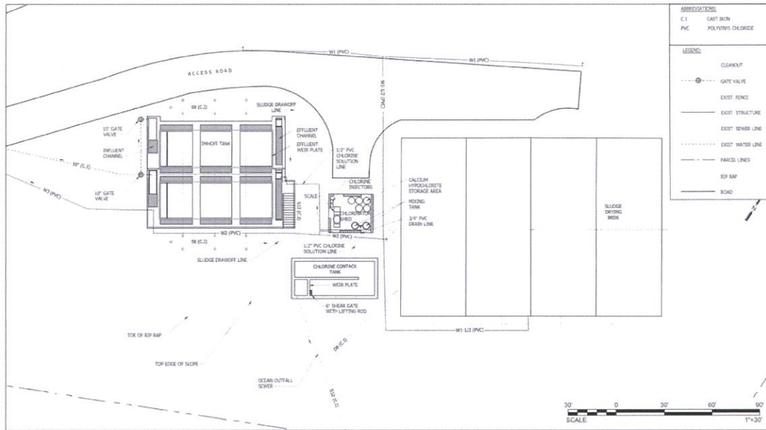
Existing Colonia WWTP Facilities
